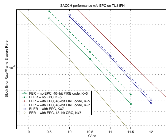
Figure 4. SACCH Performance with and without EPC
